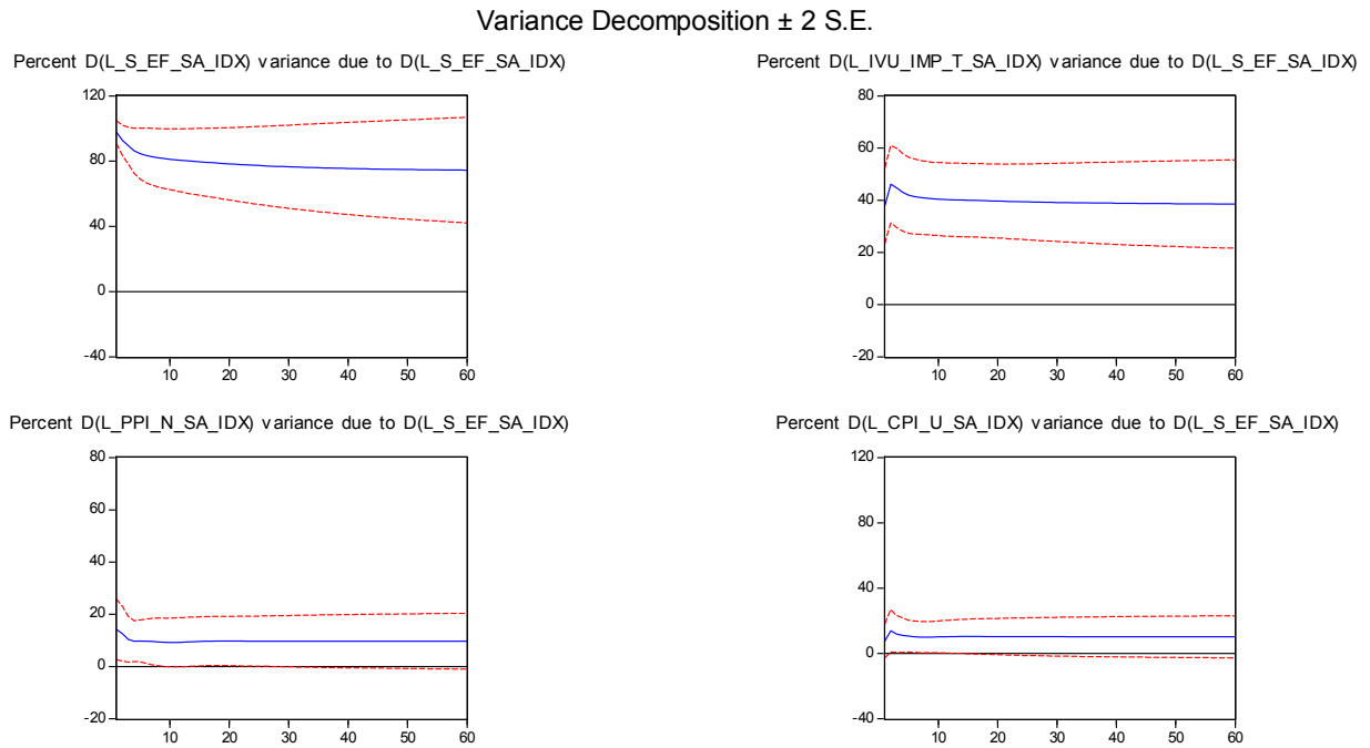
Figure 3 - Variance Decomposition
